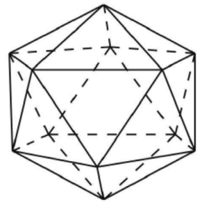
Figure 1 This is a Icosahedron
